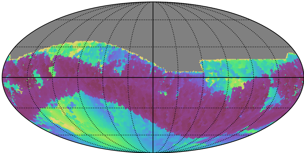
baseline_v3.5_10yrs All sky i band: Min solarElong
