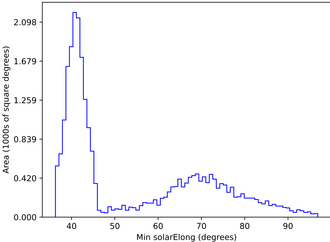
baseline_v3.5_10yrs All sky i band: Min solarElong
