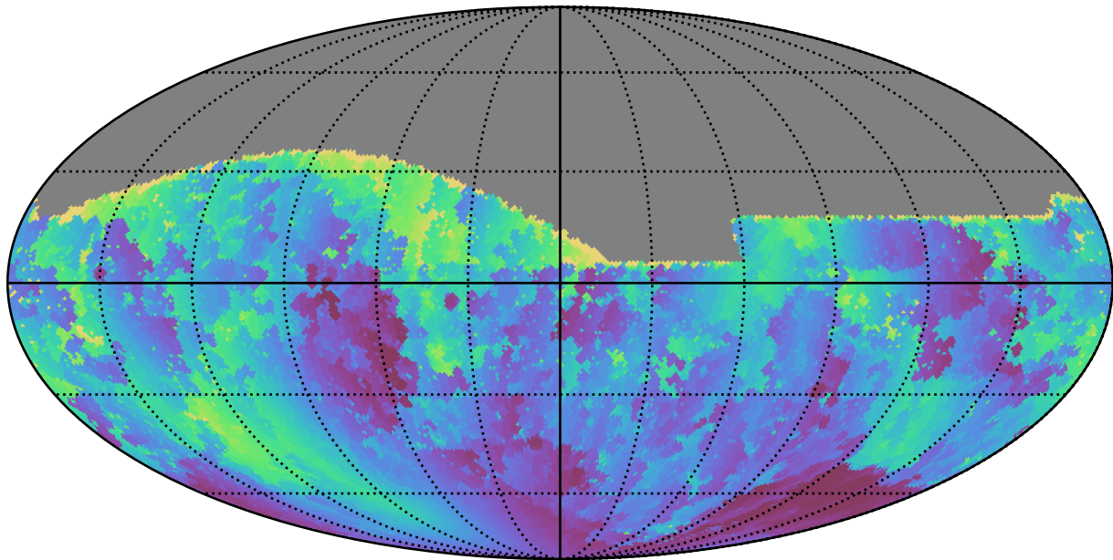
baseline_v3.5_10yrs All sky g band: Min solarElong
