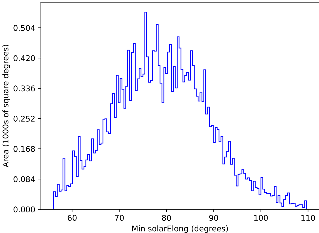
baseline_v3.5_10yrs All sky g band: Min solarElong
