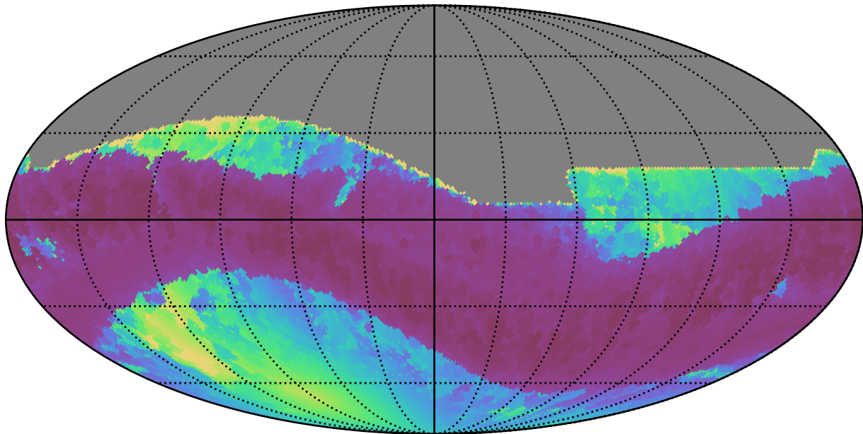
baseline_v3.5_10yrs All sky all bands: Min solarElong
