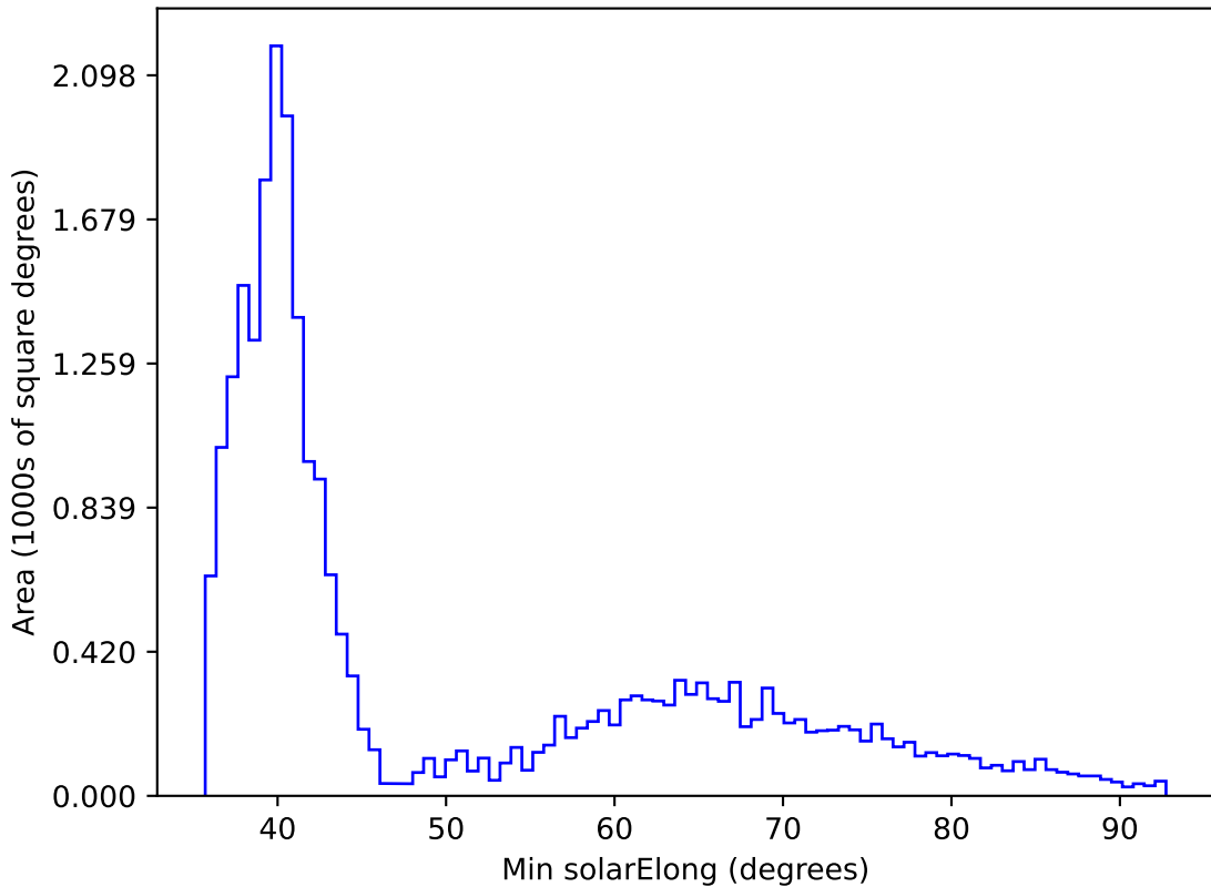
baseline_v3.5_10yrs All sky all bands: Min solarElong
