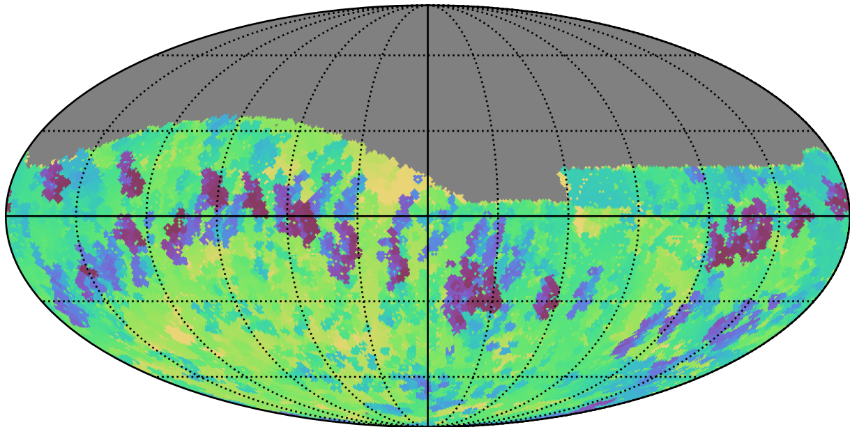
baseline_v3.5_10yrs Yr 1 z band: Min skyBrightness
