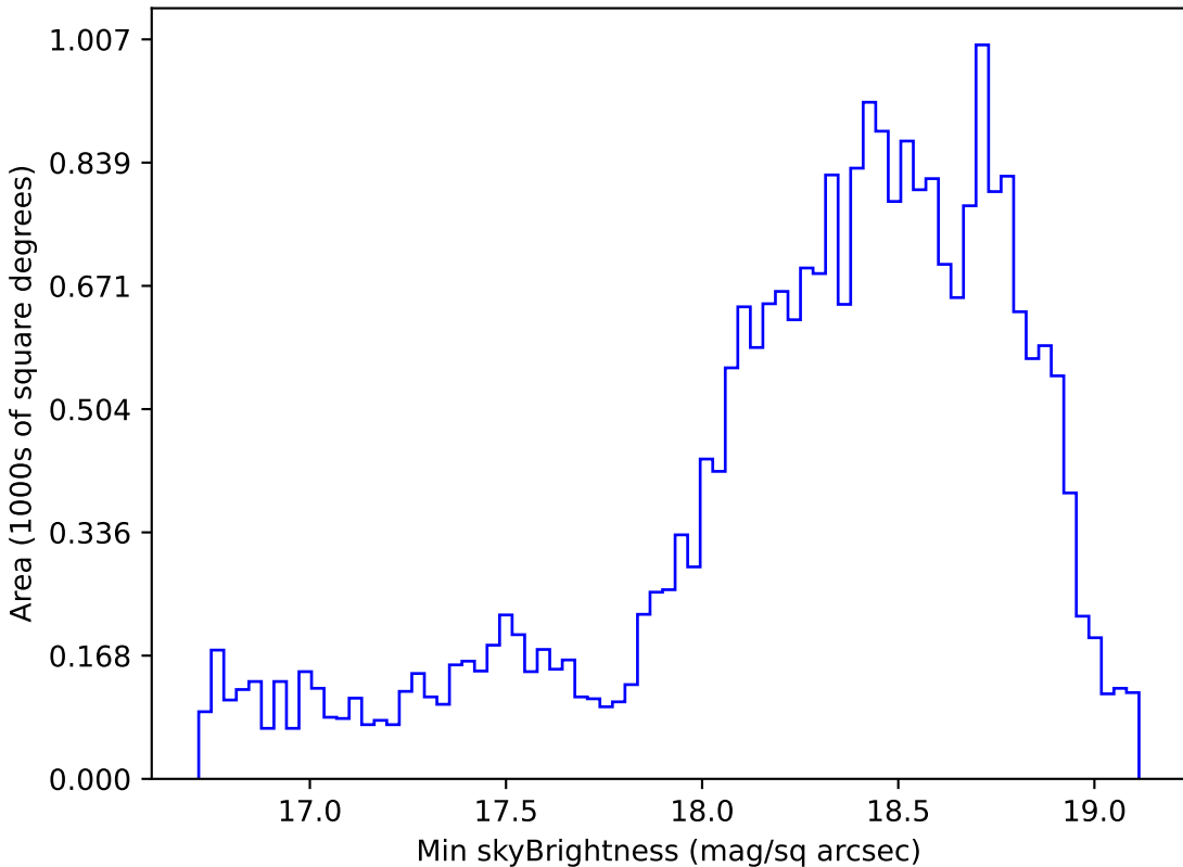
baseline_v3.5_10yrs Yr 1 z band: Min skyBrightness
