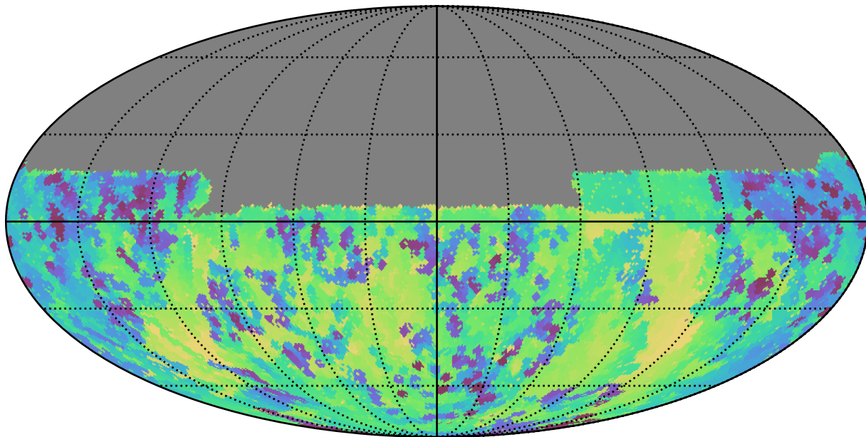
baseline_v3.5_10yrs Yr 1 y band: Min skyBrightness
