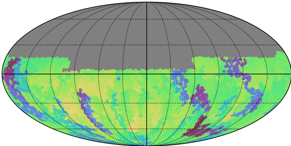
baseline_v3.5_10yrs Yr 1 u band: Min skyBrightness
