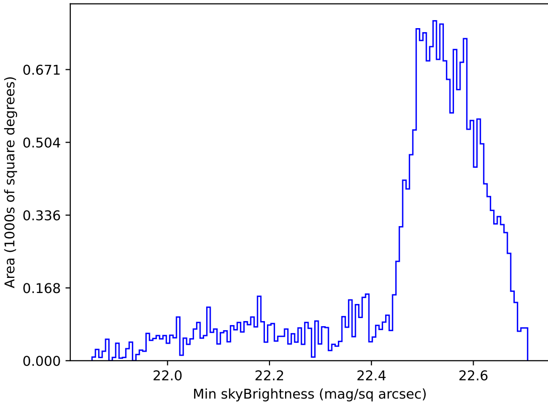
baseline_v3.5_10yrs Yr 1 u band: Min skyBrightness
