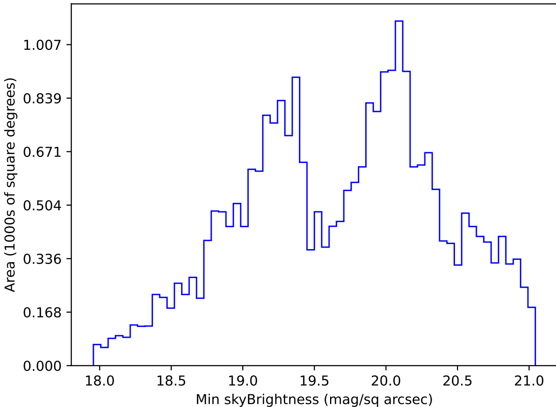
baseline_v3.5_10yrs Yr 1 r band: Min skyBrightness
