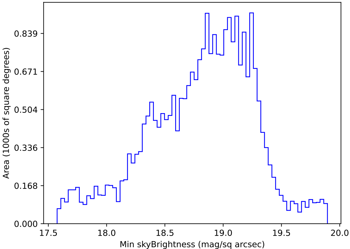
baseline_v3.5_10yrs Yr 1 i band: Min skyBrightness
