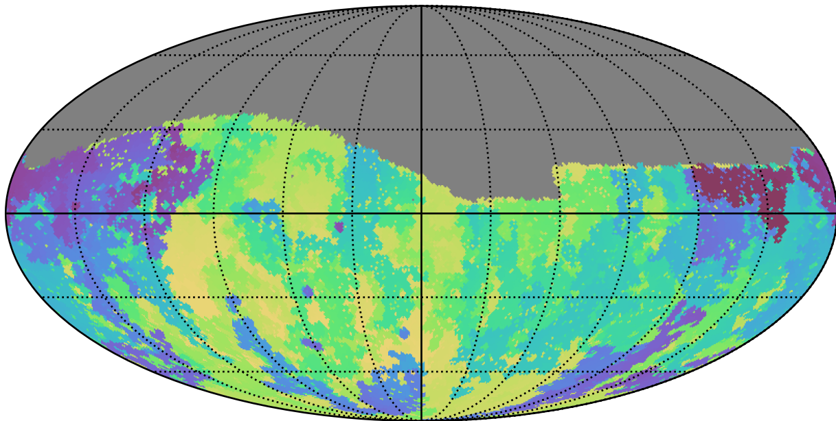
baseline_v3.5_10yrs Yr 1 g band: Min skyBrightness
