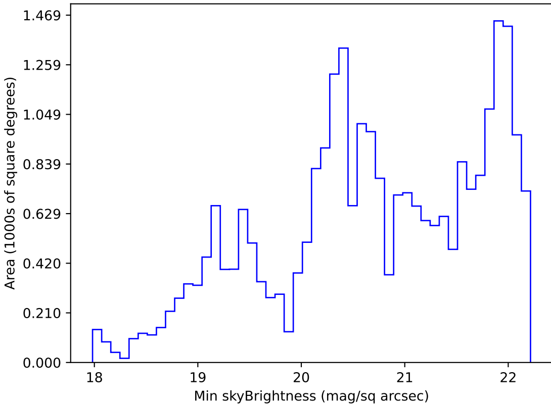
baseline_v3.5_10yrs Yr 1 g band: Min skyBrightness
