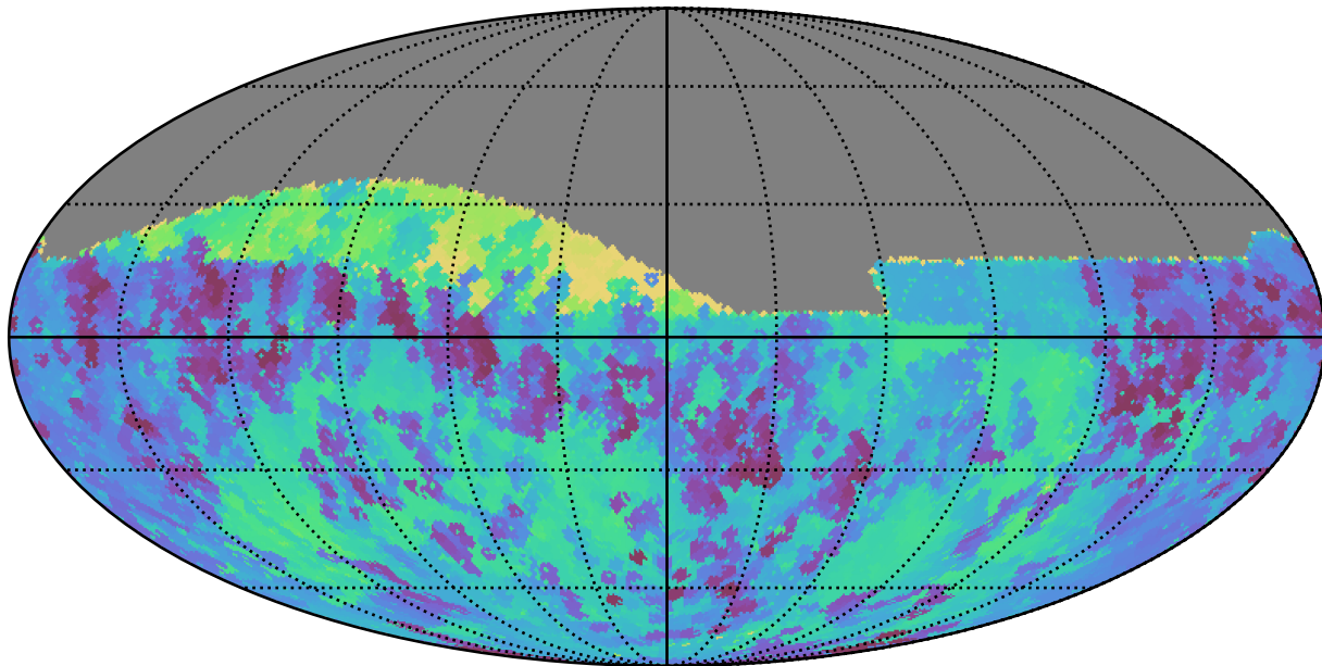
baseline_v3.5_10yrs Yr 1 all bands: Min skyBrightness
