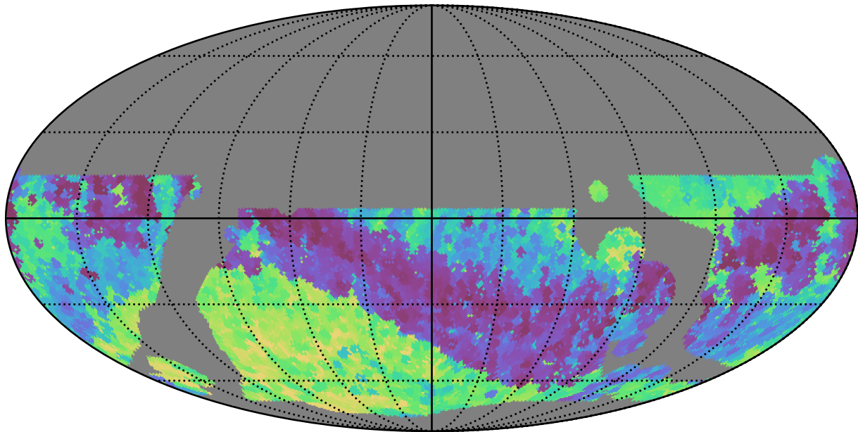
baseline_v3.5_10yrs WFD z band: Min skyBrightness
