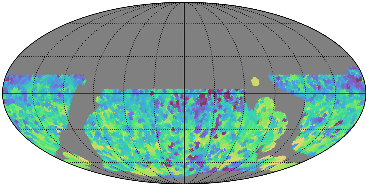
baseline_v3.5_10yrs WFD y band: Min skyBrightness
