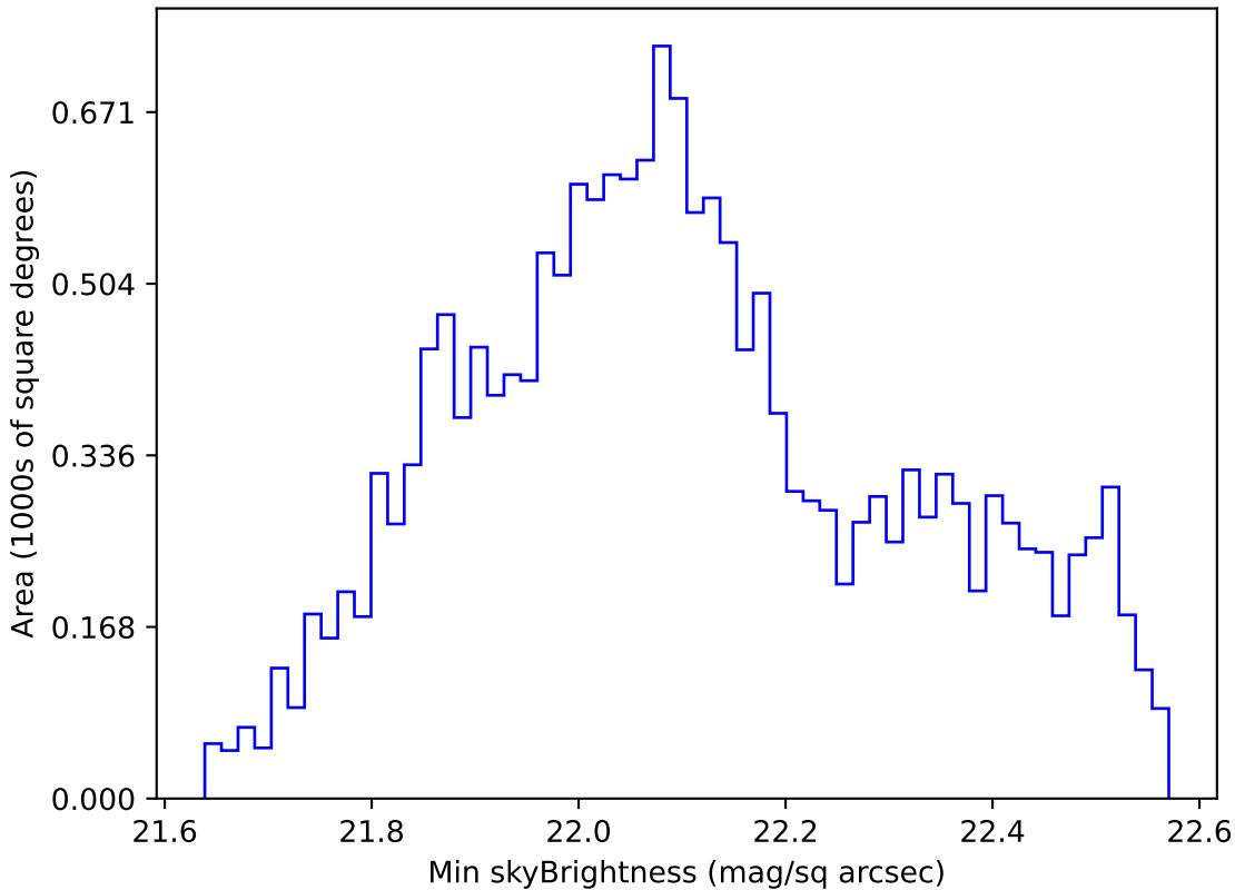
baseline_v3.5_10yrs WFD u band: Min skyBrightness
