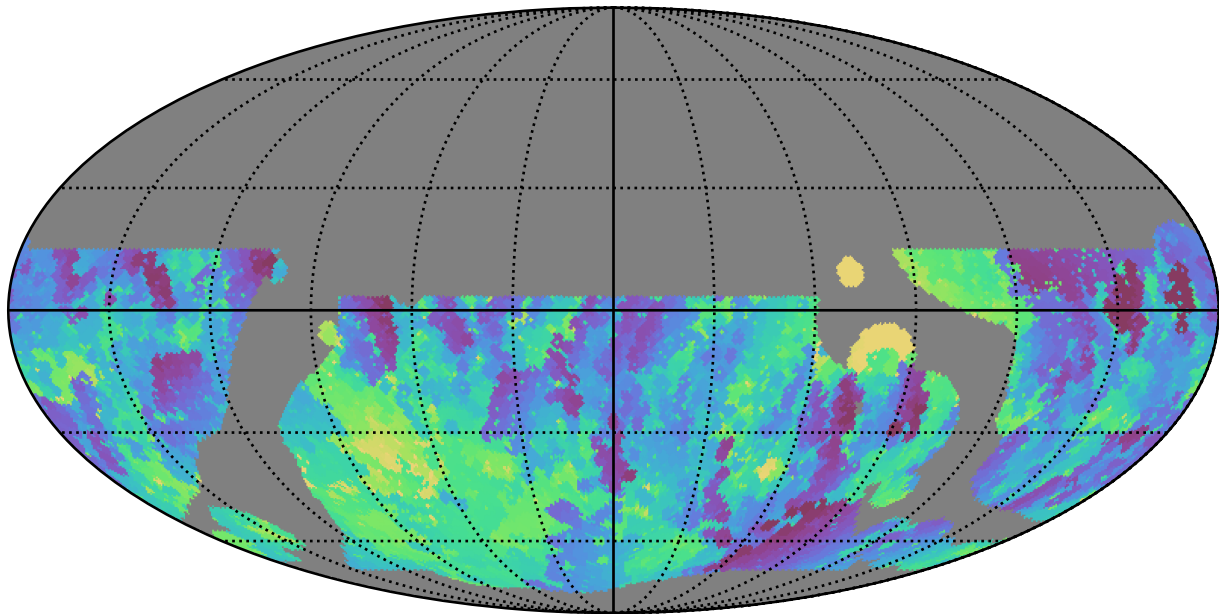
baseline_v3.5_10yrs WFD r band: Min skyBrightness
