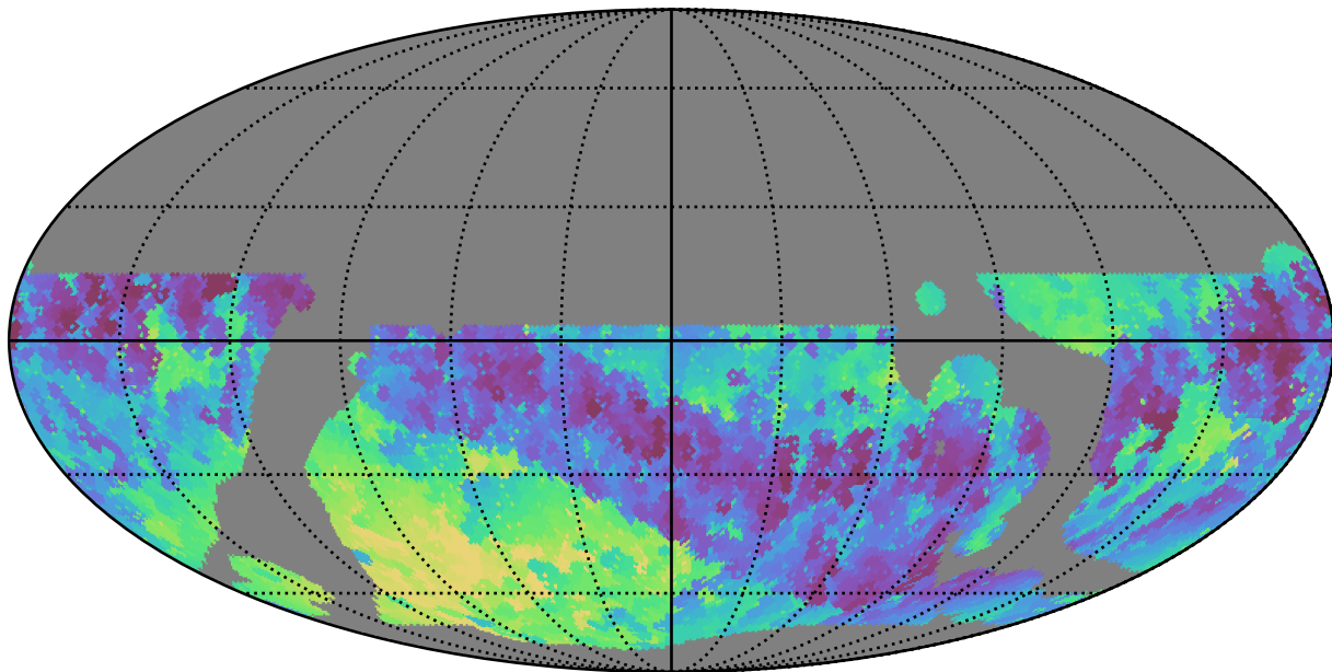
baseline_v3.5_10yrs WFD i band: Min skyBrightness
