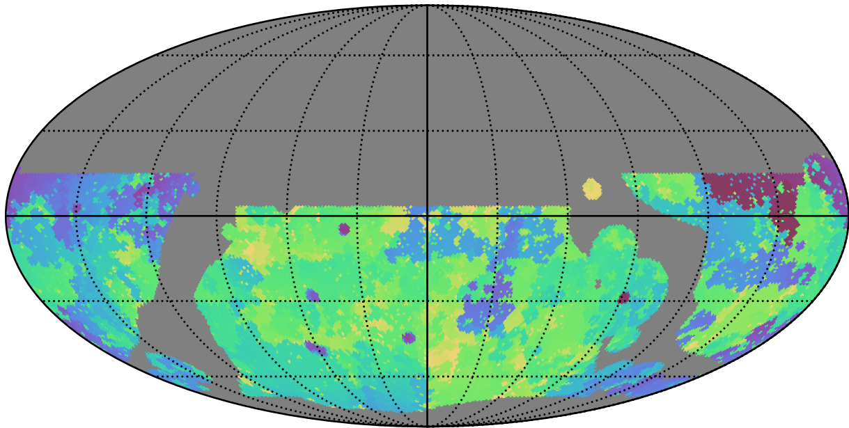
baseline_v3.5_10yrs WFD g band: Min skyBrightness
