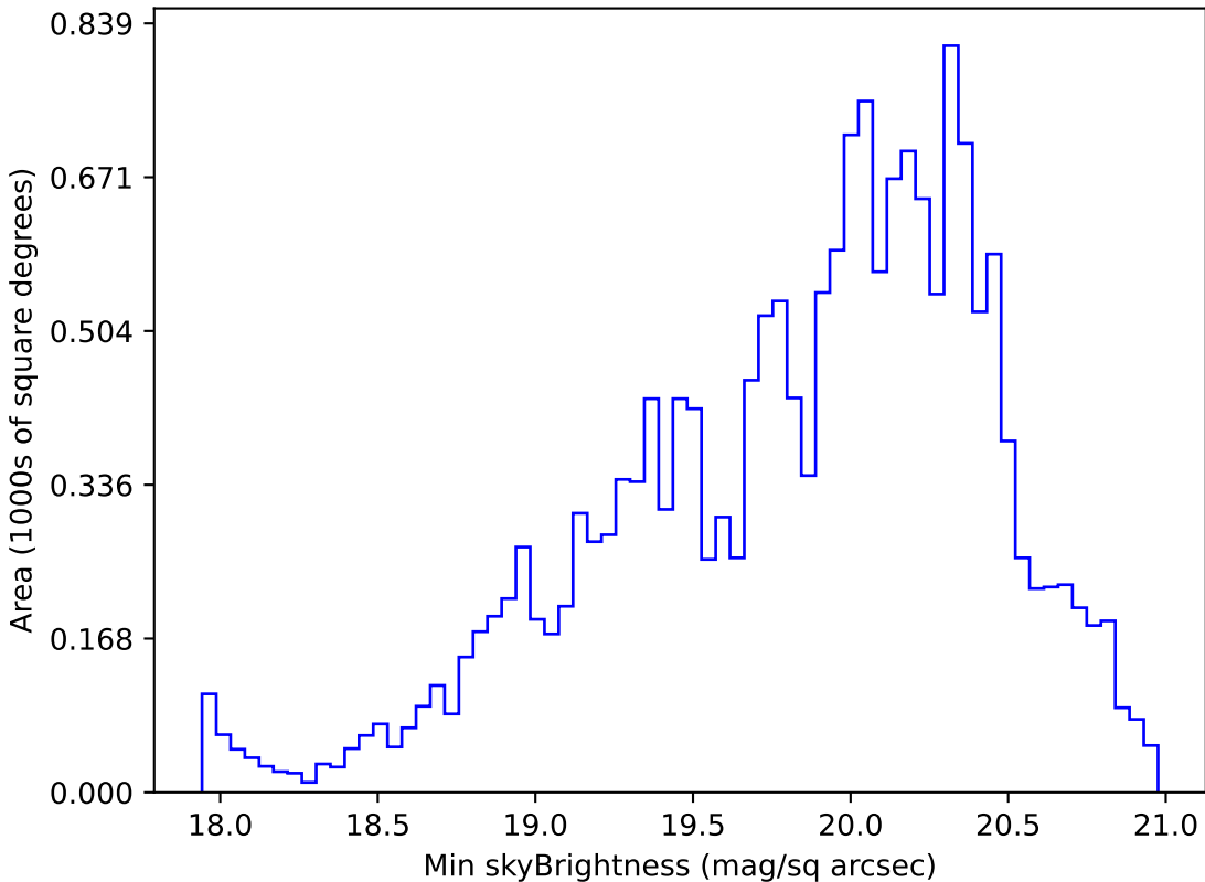
baseline_v3.5_10yrs WFD g band: Min skyBrightness
