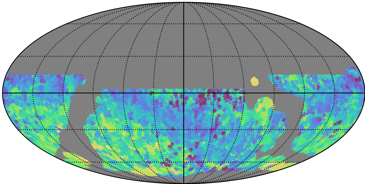
baseline_v3.5_10yrs WFD all bands: Min skyBrightness
