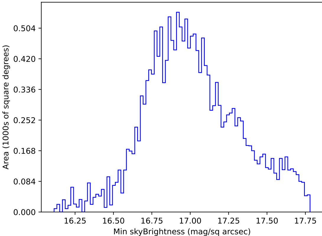
baseline_v3.5_10yrs WFD all bands: Min skyBrightness
