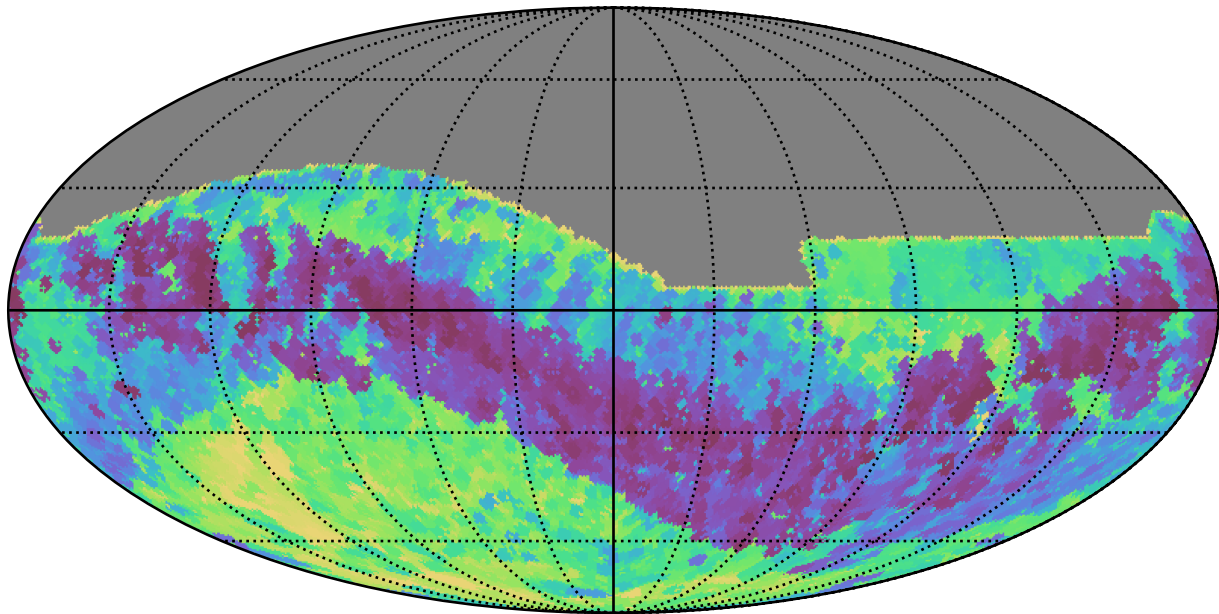
baseline_v3.5_10yrs All sky z band: Min skyBrightness
