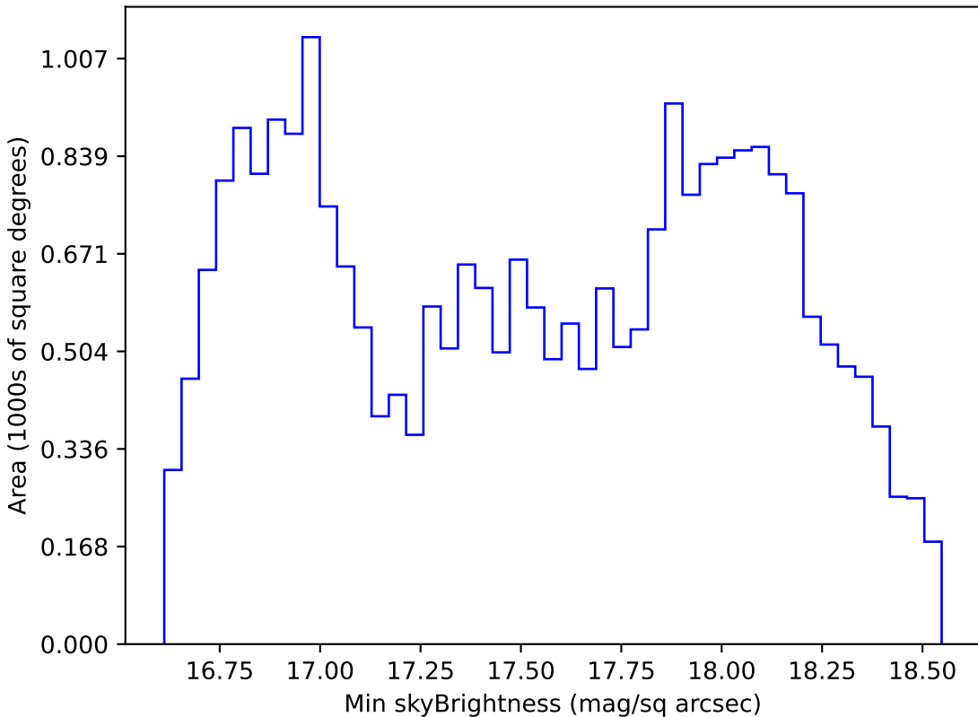
baseline_v3.5_10yrs All sky z band: Min skyBrightness
