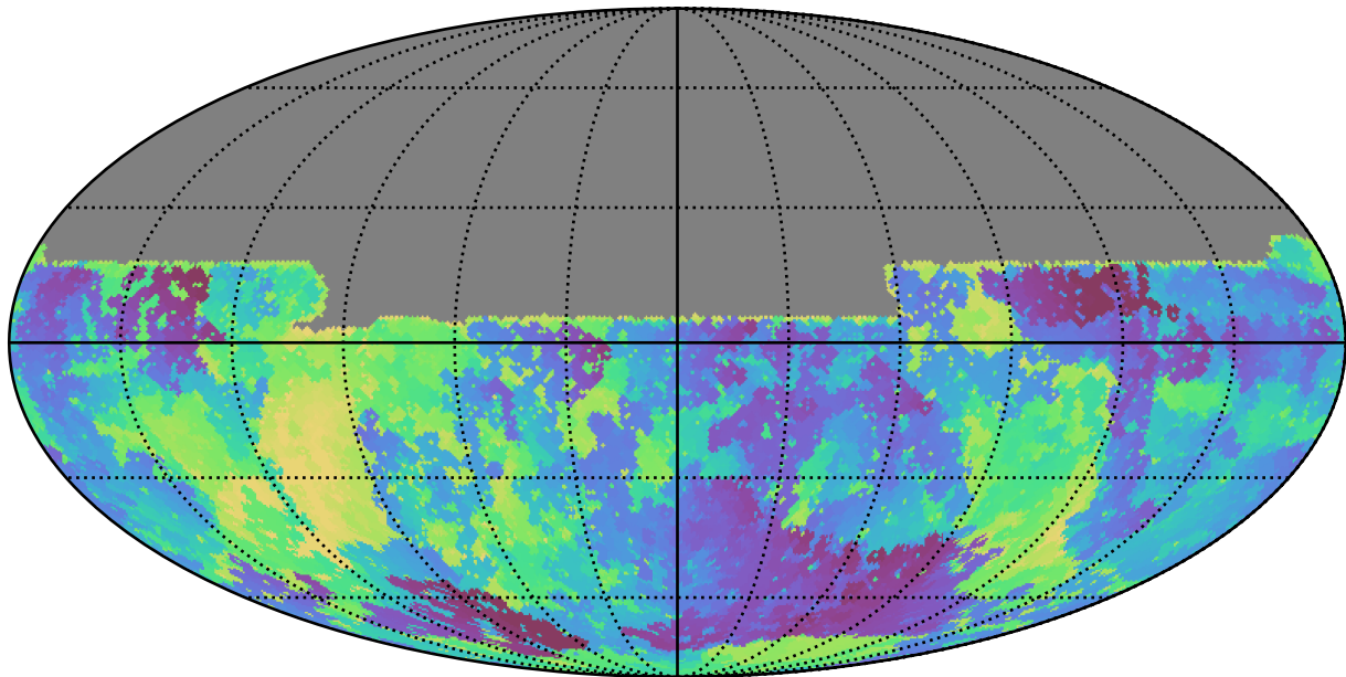
baseline_v3.5_10yrs All sky u band: Min skyBrightness
