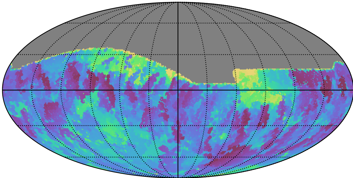
baseline_v3.5_10yrs All sky r band: Min skyBrightness
