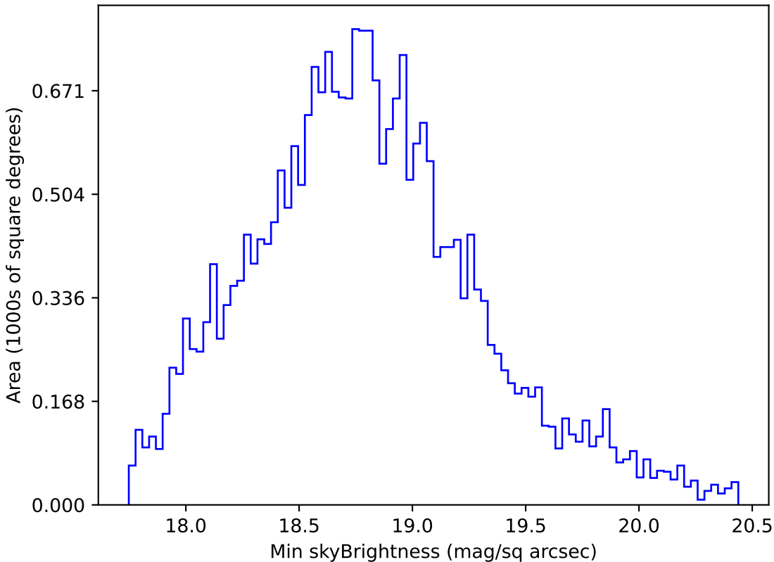
baseline_v3.5_10yrs All sky r band: Min skyBrightness
