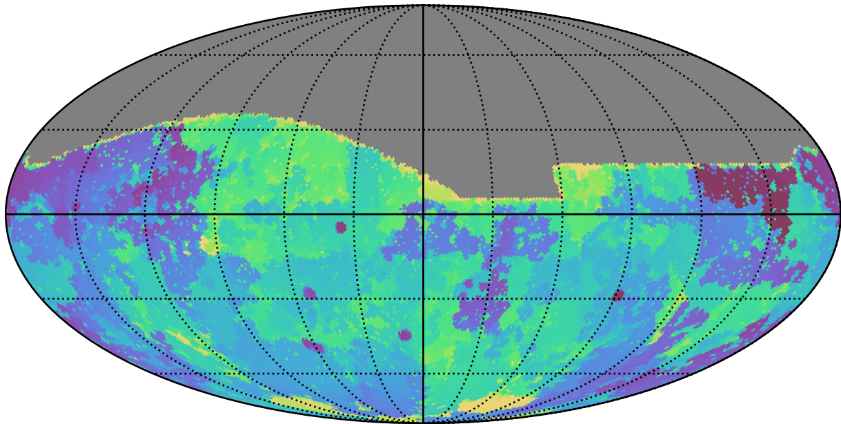
baseline_v3.5_10yrs All sky g band: Min skyBrightness
