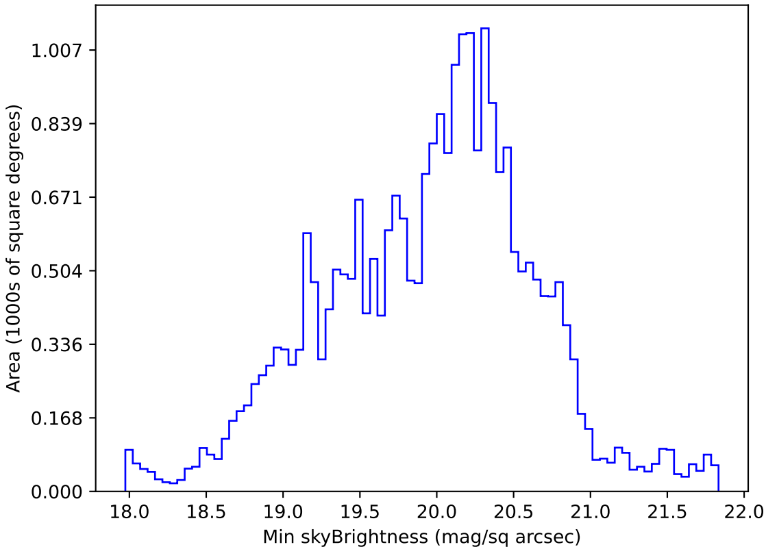
baseline_v3.5_10yrs All sky g band: Min skyBrightness
