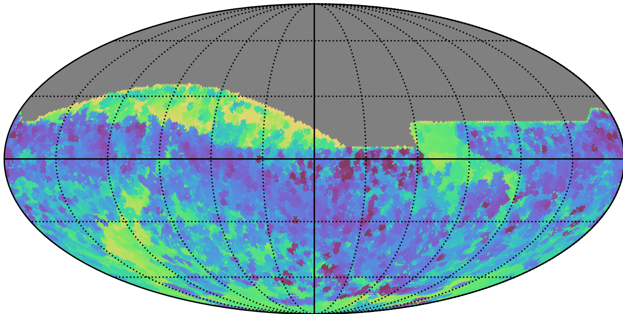
baseline_v3.5_10yrs All sky all bands: Min skyBrightness
