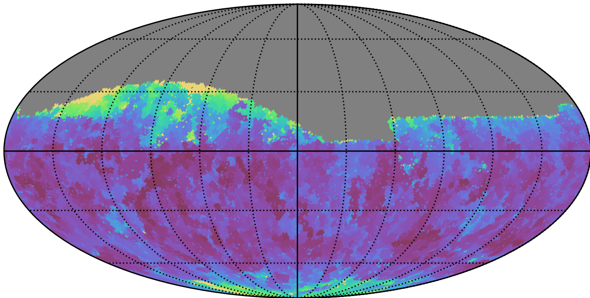
baseline_v3.5_10yrs Yr 1 z band: Min seeingGeom
