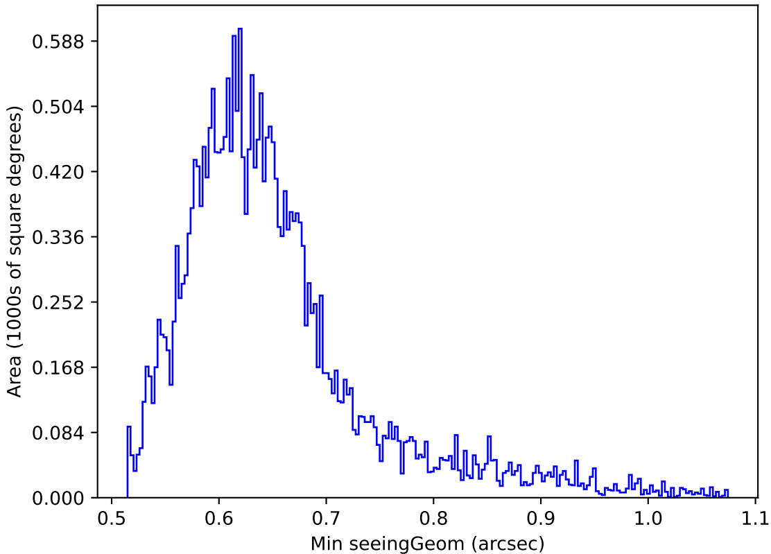
baseline_v3.5_10yrs Yr 1 z band: Min seeingGeom
