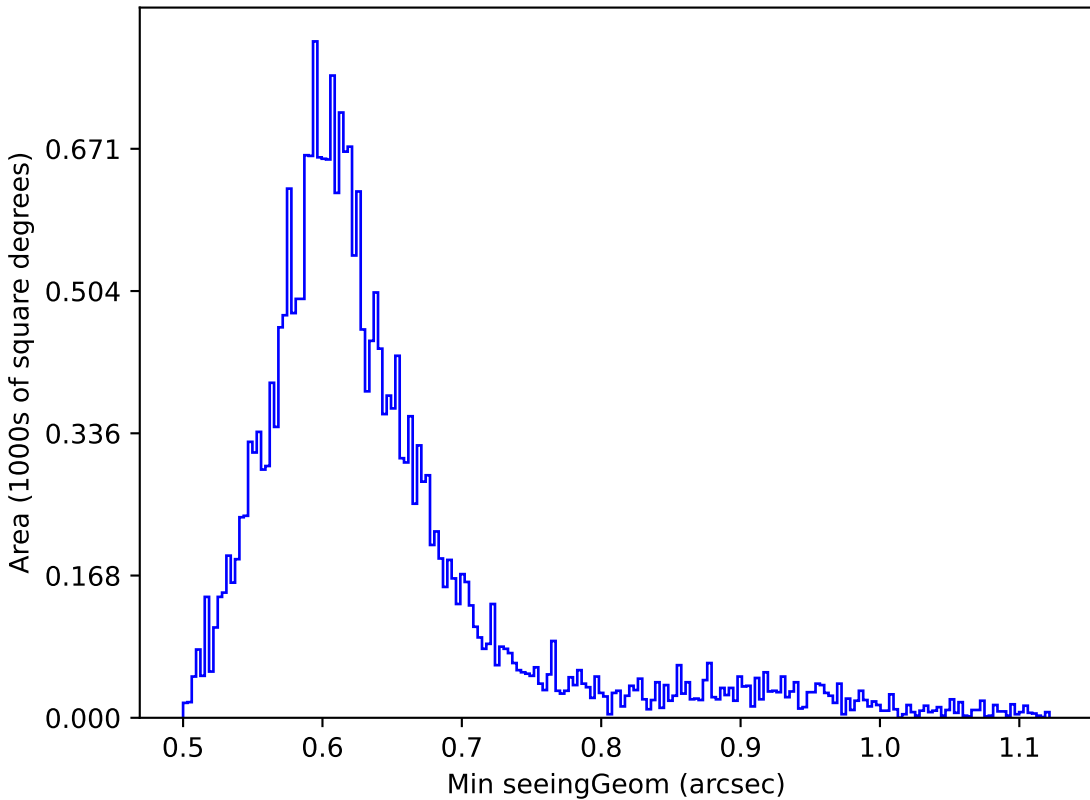
baseline_v3.5_10yrs Yr 1 r band: Min seeingGeom
