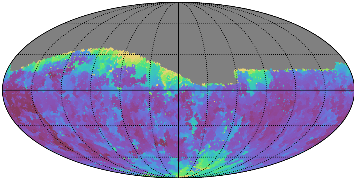
baseline_v3.5_10yrs Yr 1 g band: Min seeingGeom
