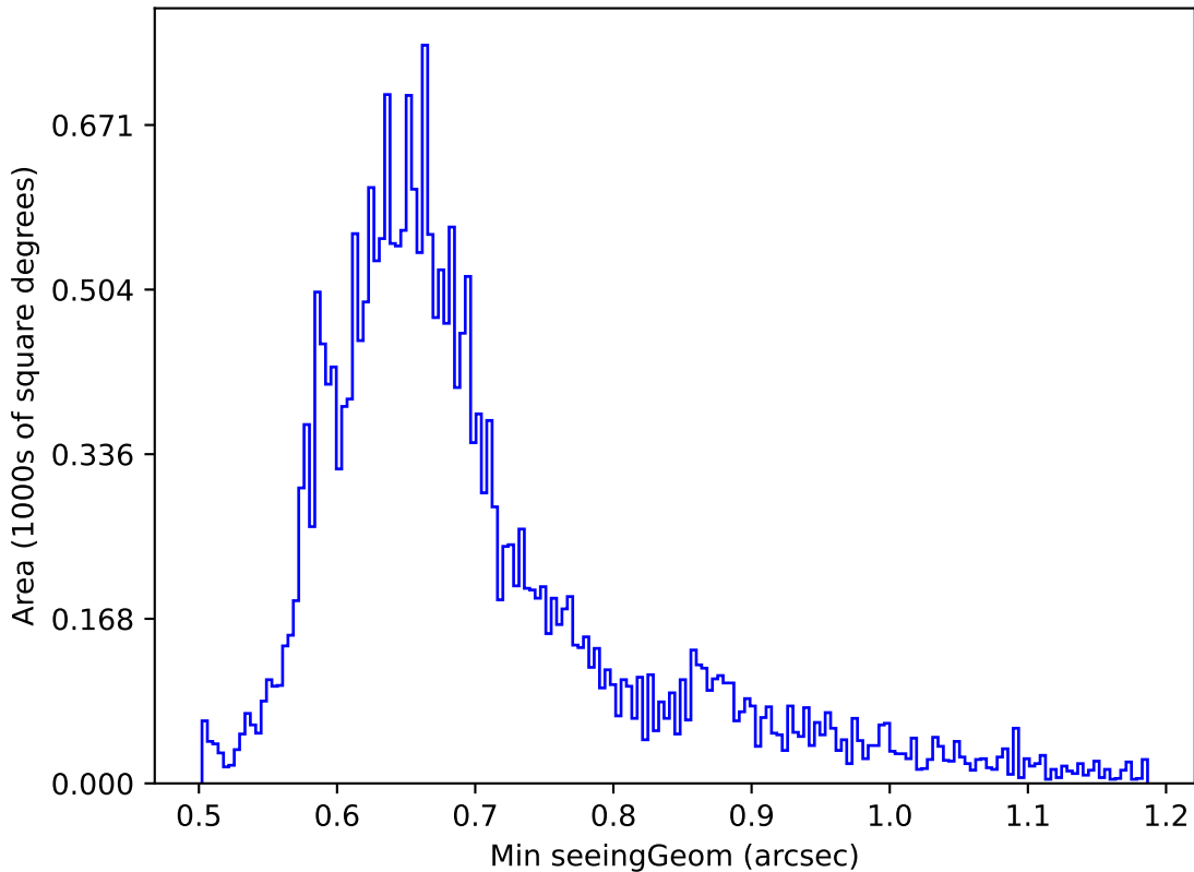
baseline_v3.5_10yrs Yr 1 g band: Min seeingGeom
