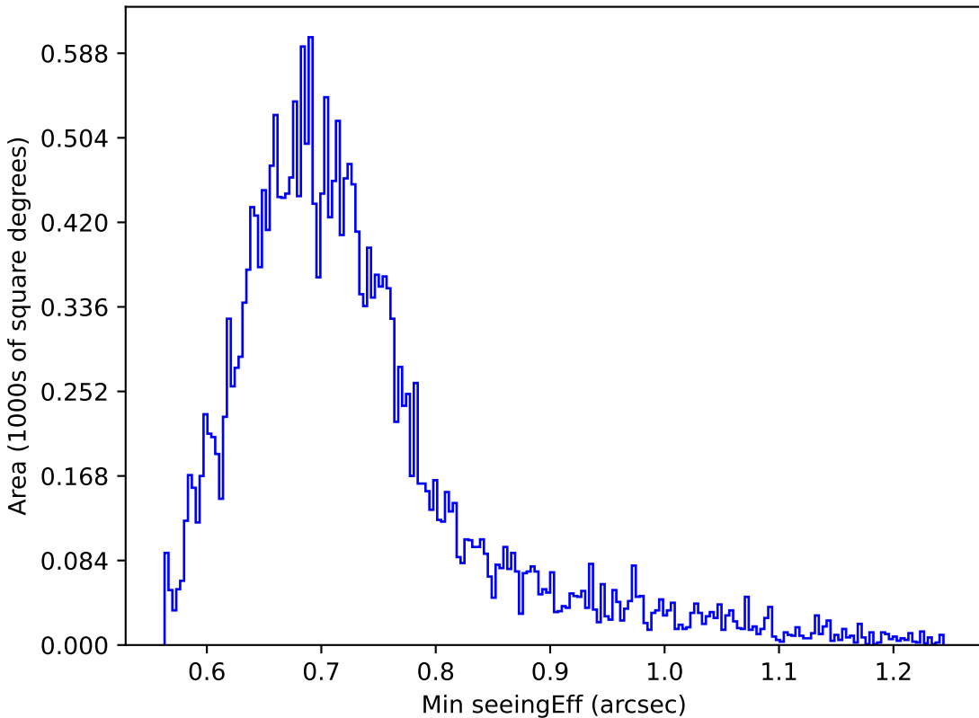
baseline_v3.5_10yrs Yr 1 z band: Min seeingEff
