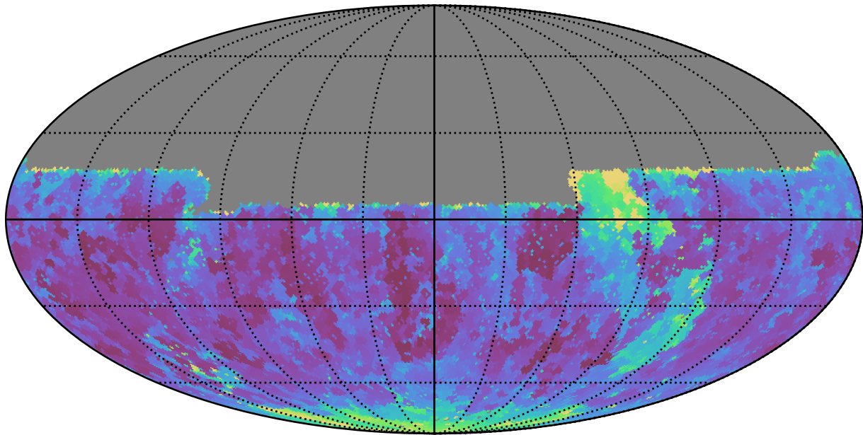
baseline_v3.5_10yrs Yr 1 y band: Min seeingEff
