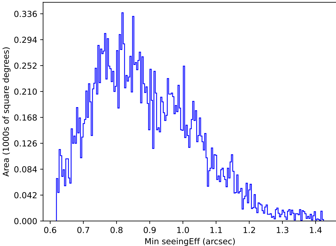
baseline_v3.5_10yrs Yr 1 u band: Min seeingEff
