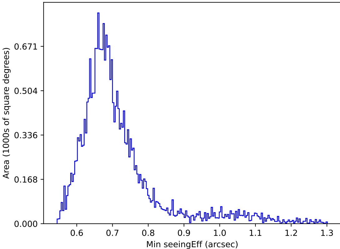
baseline_v3.5_10yrs Yr 1 r band: Min seeingEff
