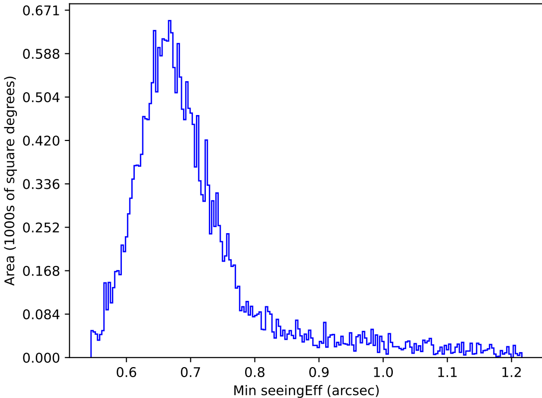
baseline_v3.5_10yrs Yr 1 i band: Min seeingEff
