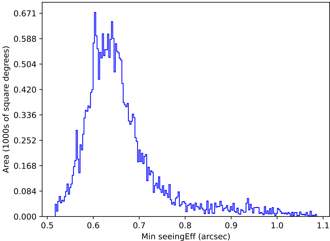
baseline_v3.5_10yrs Yr 1 all bands: Min seeingEff
