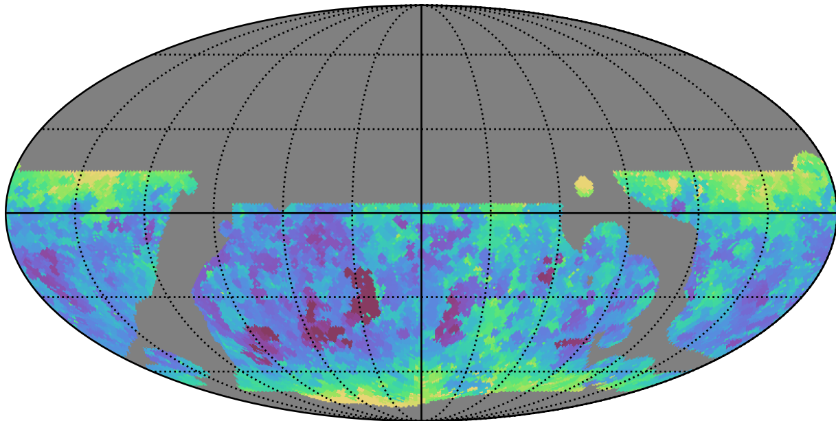
baseline_v3.5_10yrs WFD z band: Min seeingEff
