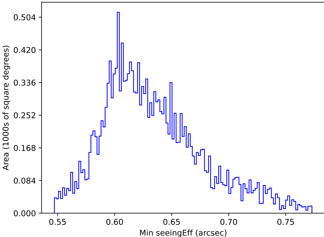
baseline_v3.5_10yrs WFD y band: Min seeingEff
