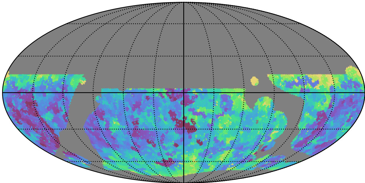
baseline_v3.5_10yrs WFD u band: Min seeingEff
