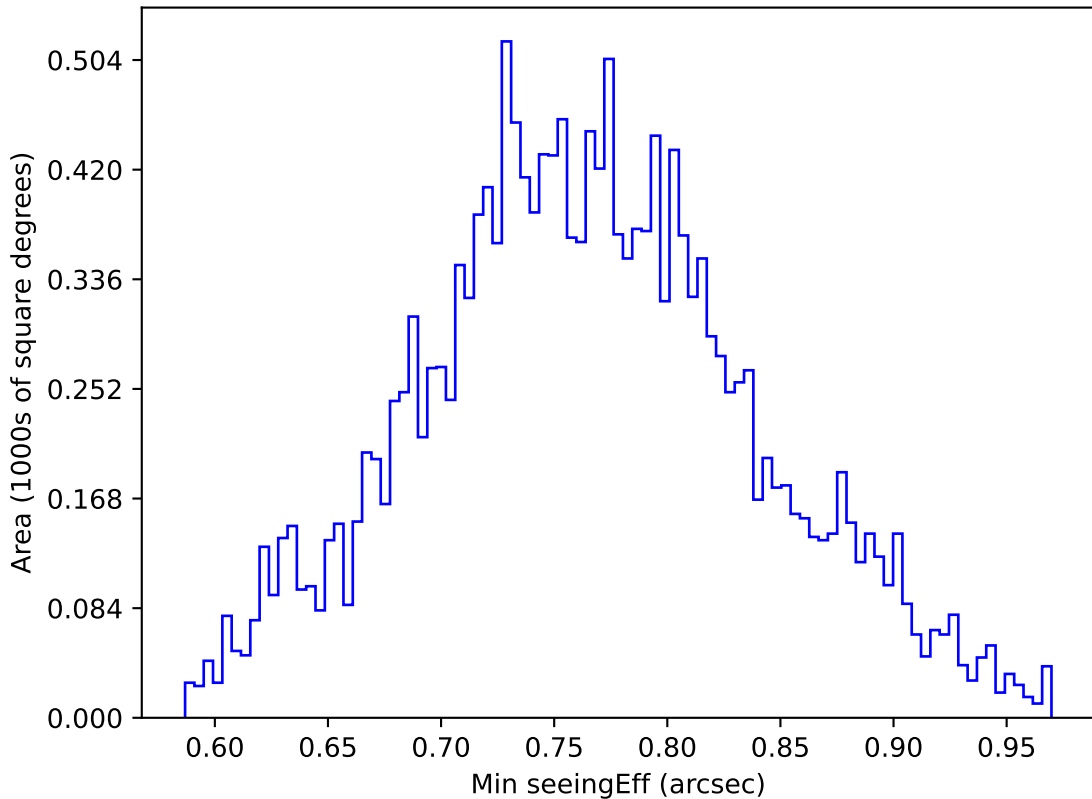
baseline_v3.5_10yrs WFD u band: Min seeingEff
