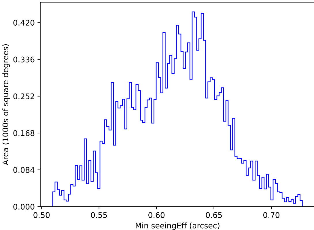
baseline_v3.5_10yrs WFD r band: Min seeingEff
