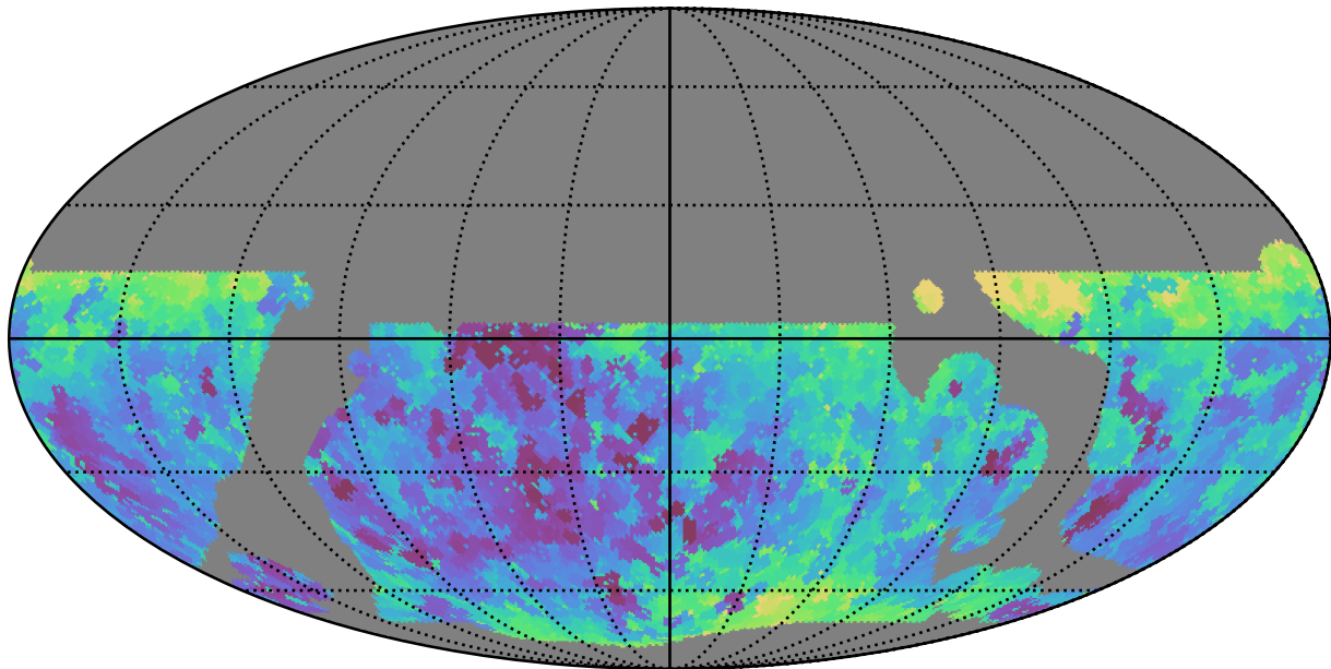
baseline_v3.5_10yrs WFD i band: Min seeingEff
